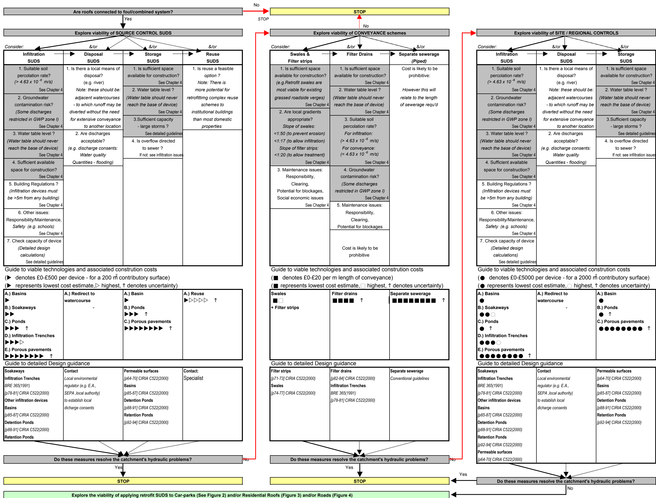
Figure 1 Proposed decision-making flowchart for the design of retrofit SUDS (Institutional Roofs)
